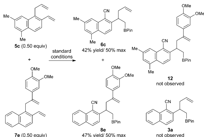
Scheme 5. Mechanistic studies.
